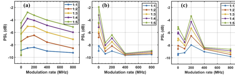
Fig. 7. The PSL of the cross-correlation results of the original 200 MHz chaotic signal with the interference of (a) chaotic wave, (b) square wave, (c) sine wave signal at different modulation rates and SINR.
